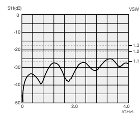
Return loss for TNP-C3
