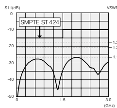
Return loss for NCP-H8HD
