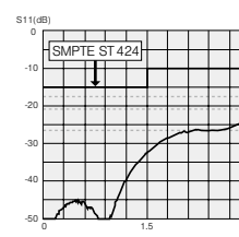
Return loss for BCJ-FPLV01
