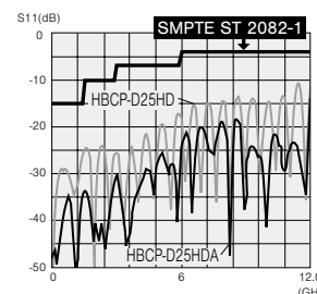
Return loss for HBCP-D25HDA, HBCP-D25HD
