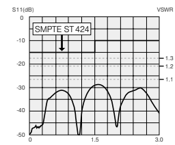
Return loss for BCP-B5F
