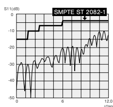
Return Loss Interface to Termination (reference)
