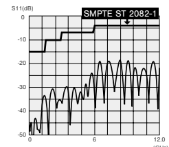
Return loss for BCP-D55UHD
