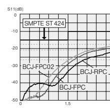
Return loss for BCJ-FPC, BCJ-FPC02, BCJ-RPC
