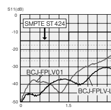
Return loss for BCJ-FPLV-L
