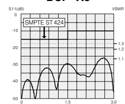
Return loss for BCP-A3
