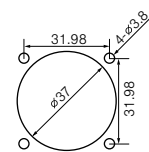
Panel Hole Dimensions (Mounting screw M3 × 4 pcs)
